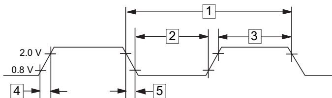
FIGURE 5 – CLOCK INPUT TIMING DIAGRAM
